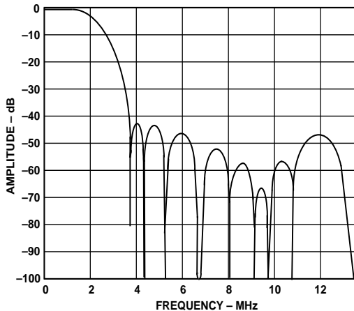
Figure 10. NTSC UV Filter
