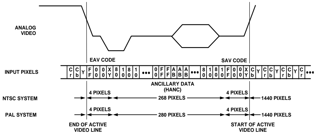
Figure 13. Timing Mode 0 (Slave Mode)
