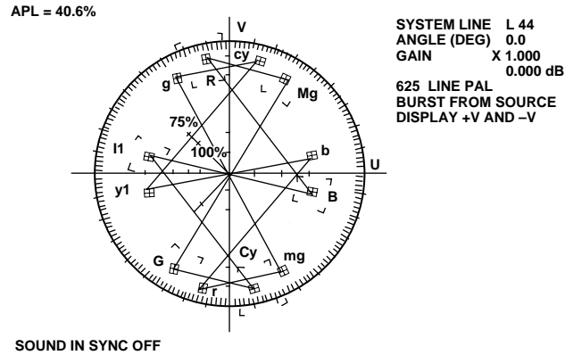
Figure 62. Vectorscope Measurements (PAL)
