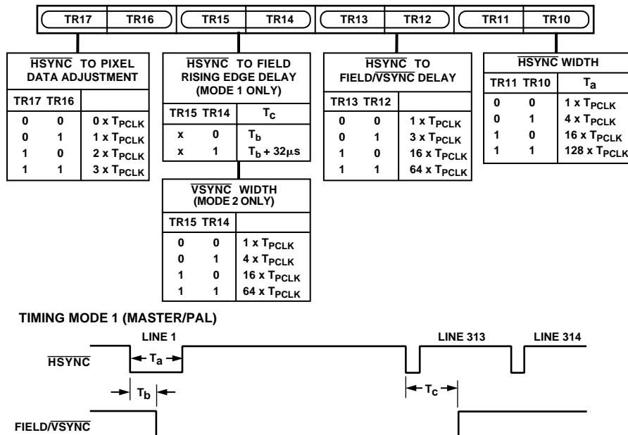
Figure 37. Timing Register 1
