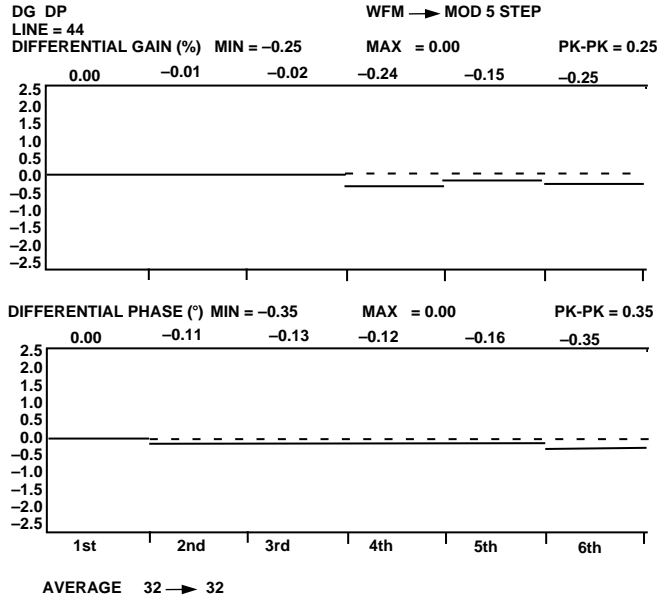
Figure 61. Differential Phase and Gain Measurements (PAL)
