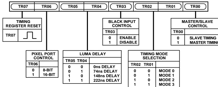
Figure 34. Timing Register 0
