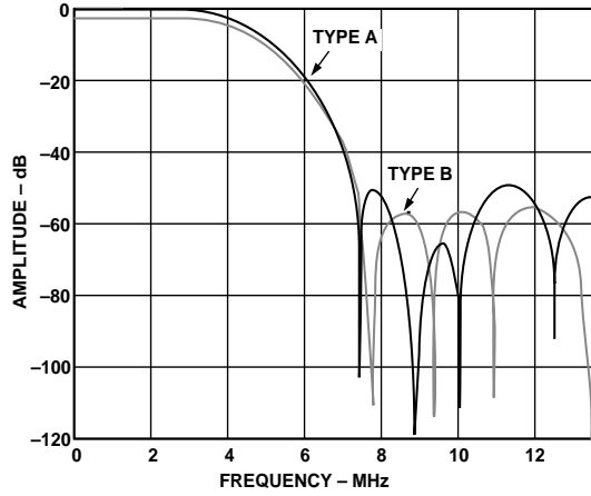
Figure 5. NTSC Low-Pass Filter
