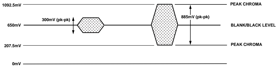
Figure 54. PAL Chroma Video Levels
