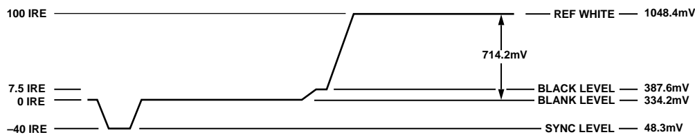
Figure 45. NTSC Luma Video Levels
