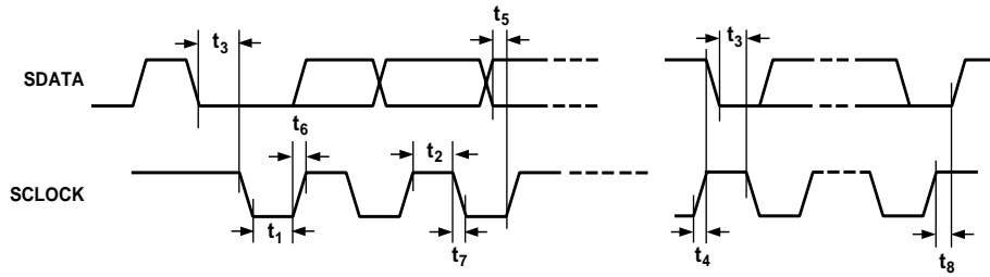
Figure 1. MPU Port Timing Diagram
