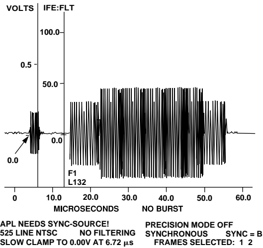
Figure 58. 100/75% Color Bars NTSC (Chrominance Only)
