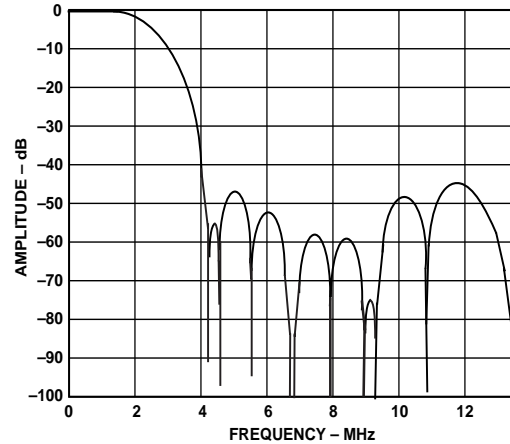
Figure 11. PAL UV Filter
