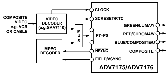
Figure 12. RTC Connections
