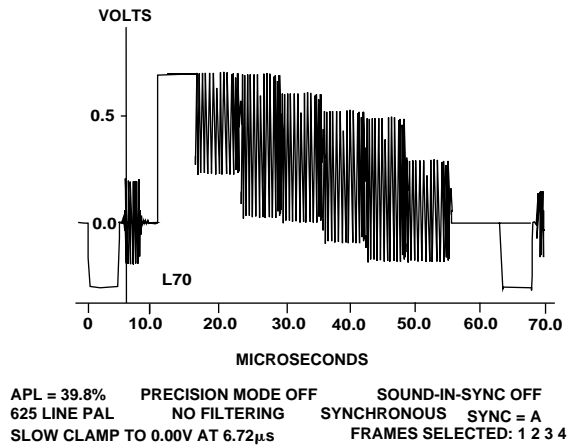
Figure 60. 100/75% Color Bars PAL
