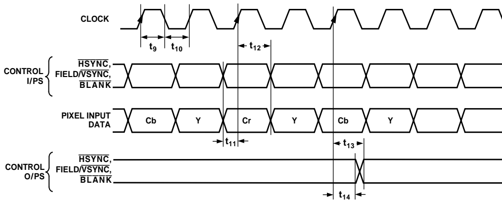
Figure 2. Pixel and Control Data Timing Diagram
