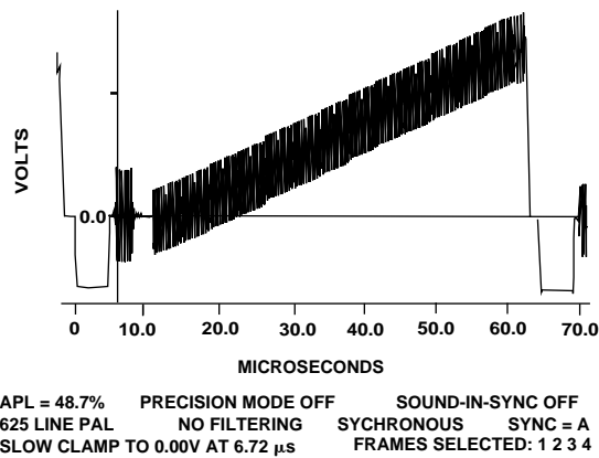
Figure 63. Modulated Ramp Measurements (PAL)
