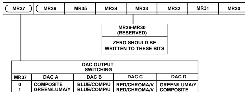
Figure 40. Mode Register 3
