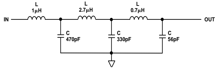
Figure 56. Output Filter
