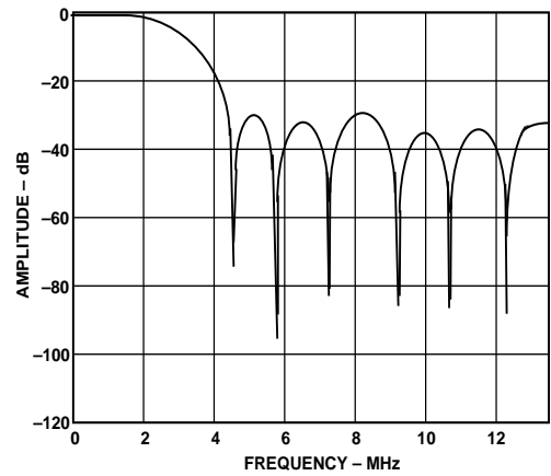
Figure 8. PAL Notch Filter
