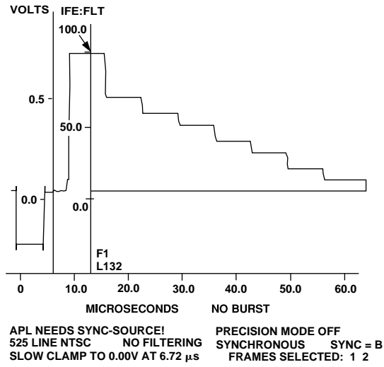
Figure 59. 100/75% Color Bars NTSC (Luminance Only)
