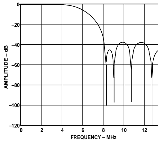
Figure 9. NTSC/PAL Extended Mode Filter
