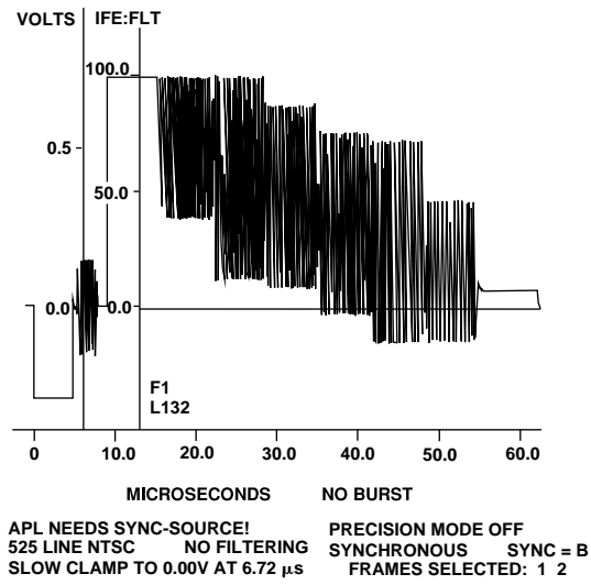
Figure 57. 100/75% Color Bars NTSC
