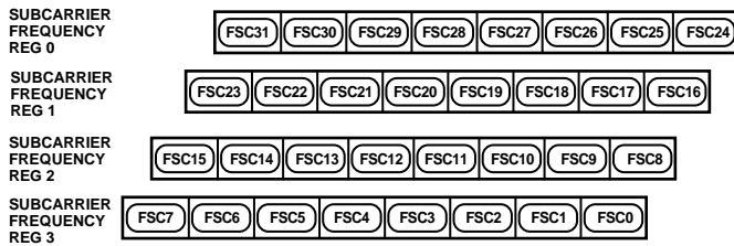
Figure 33. Subcarrier Frequency Register
