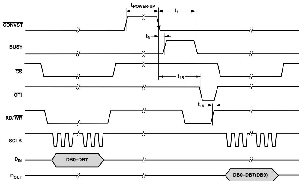
Figure 15. Mode 2 Operation
