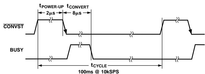
Figure 16. Automatic Power-Down
