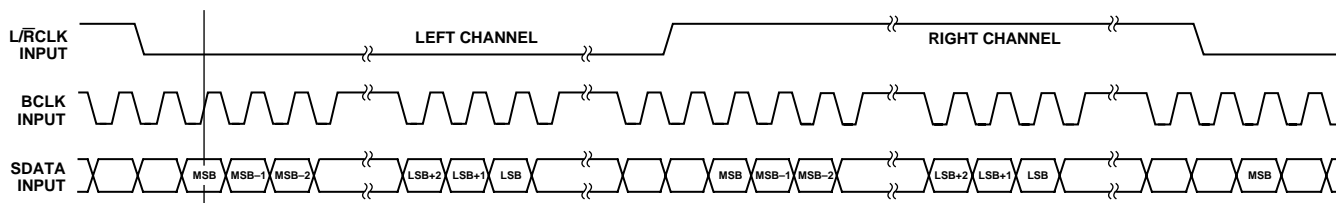
Figure 2. I²S-Justified Mode
