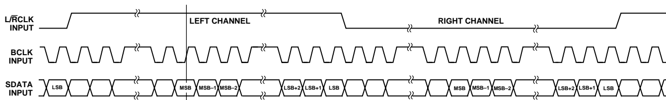
Figure 1. Right-Justified Mode
