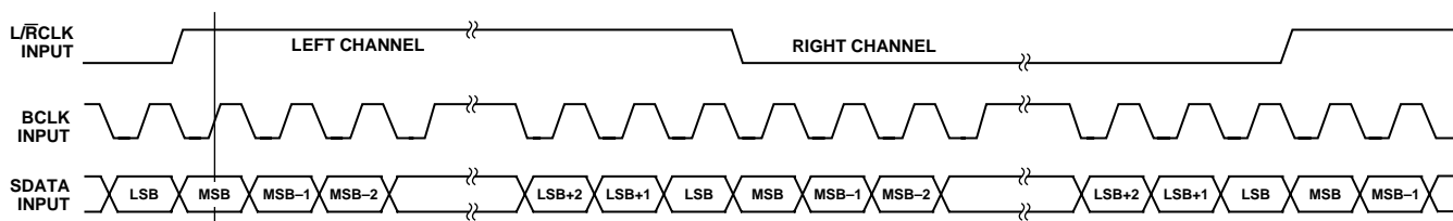
Figure 4. 32 \times F_S Packed Mode
