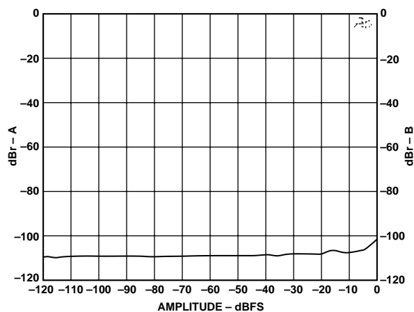
Figure 13. THD+N vs. Level at 1 kHz
