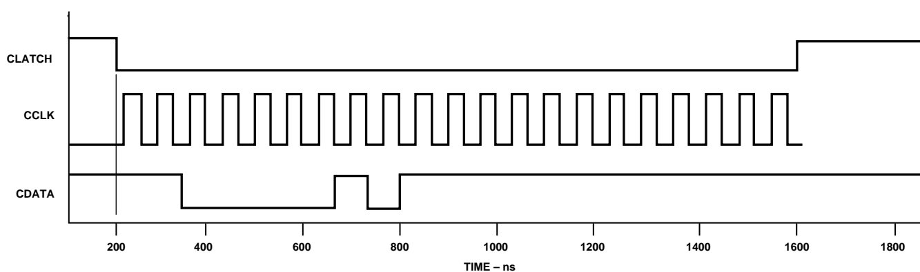
Figure 7. SPI Port Burst Mode
