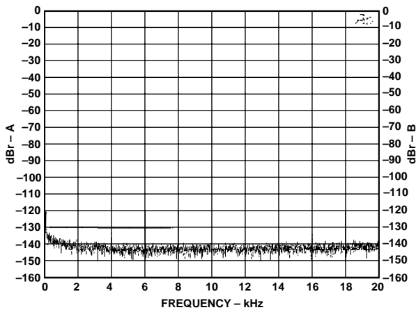
Figure 15. Noise Floor, A-Weighted (8K-Point FFT)
