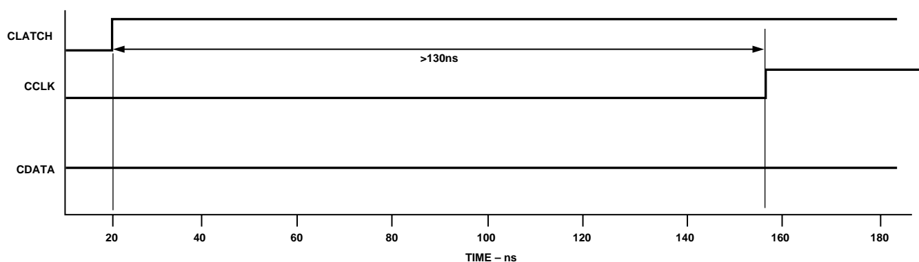
Figure 6. SPI Port Continuous CCLK Mode
