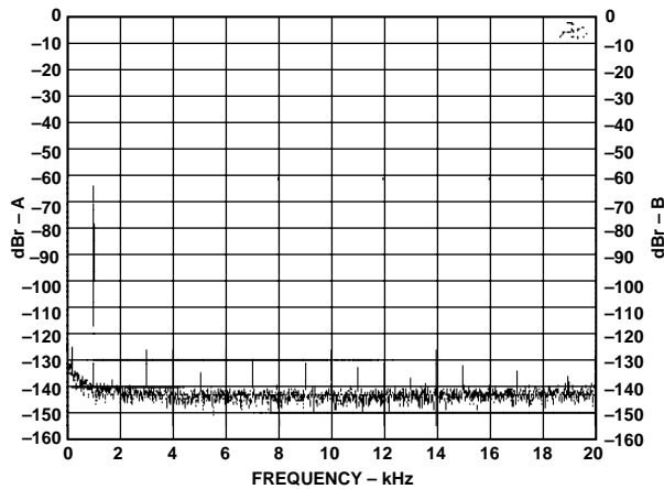
Figure 12. Dynamic Range: 1 kHz at -60 dBFS (8K Point FFT)
