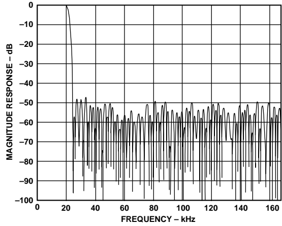
Figure 16. Digital Filter Response
