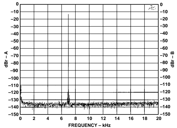
Figure 17. Two-Tone Test
