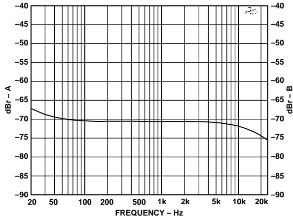
Figure 14. Power Supply Rejection to 300 mV p-p on AVDD
