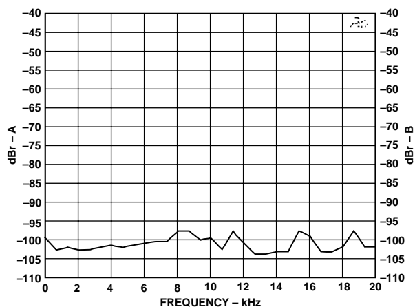
Figure 11. THD+N vs. Frequency at -0.5 dBFS
