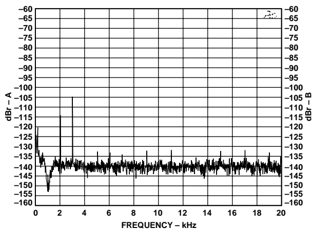
Figure 10. THD+N at 1 kHz, -0.5 dBFS (8K-Point FFT)
