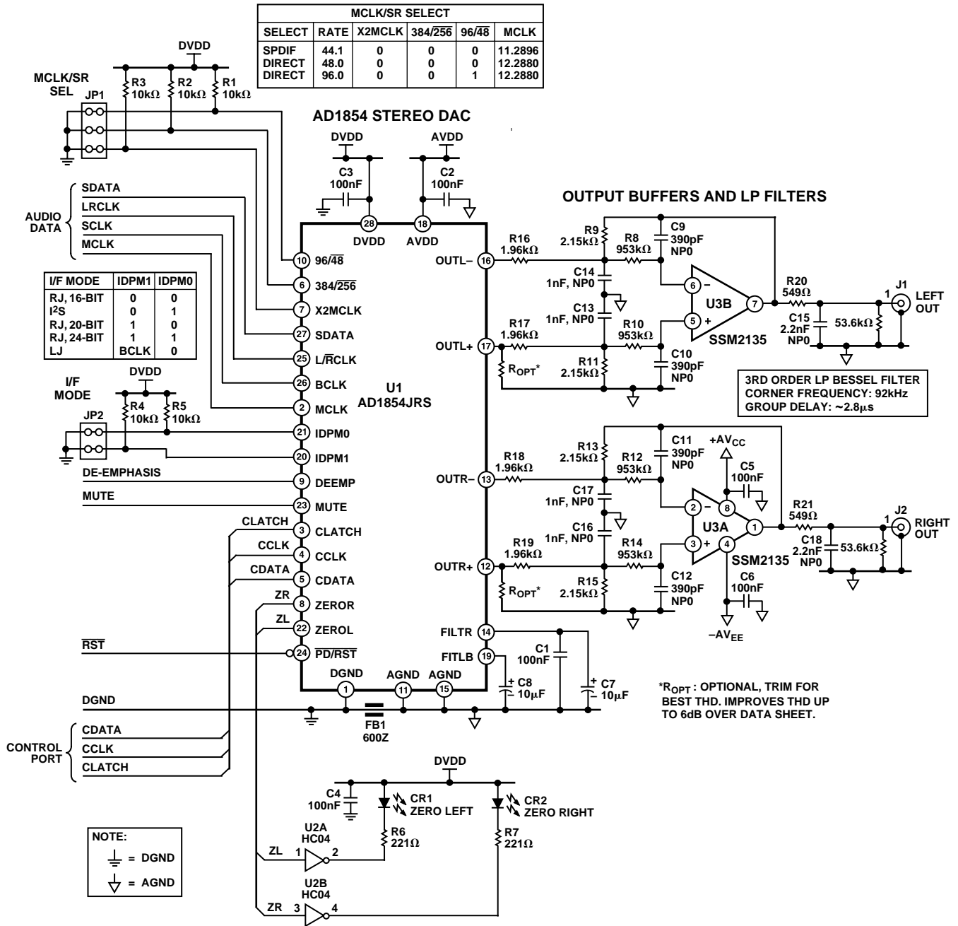
Figure 9. Evaluation Board Circuit
