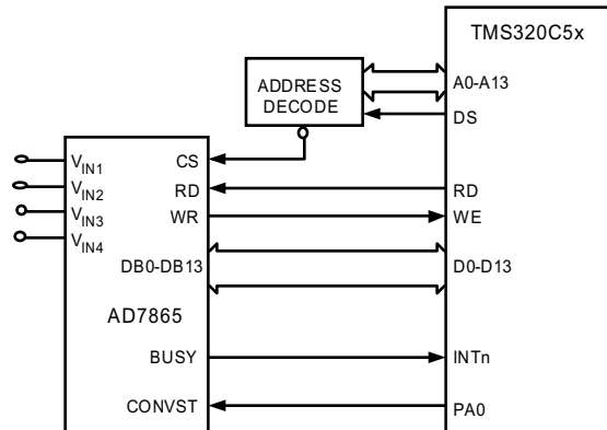
Figure 21. AD7865-TMS320C5x Interface
