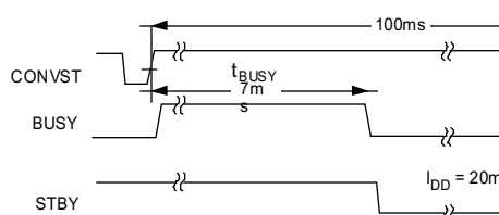
Figure 10. Power Down between Conversion Sequences
