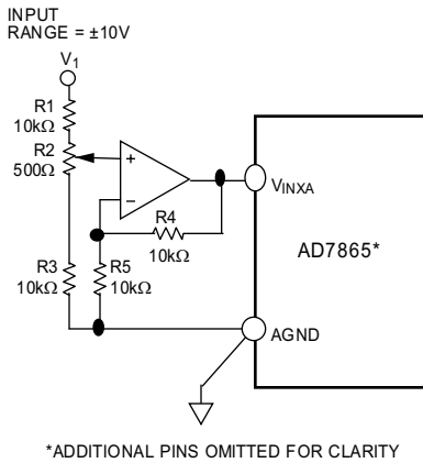
Figure 13. AD7865 Full-Scale Adjust Circuit
