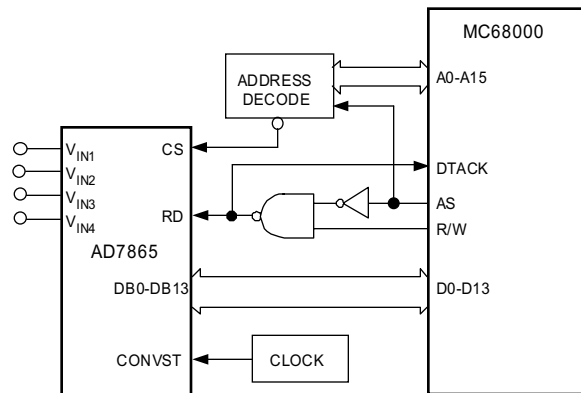
Figure 22. AD7865-MC68000 Interface
