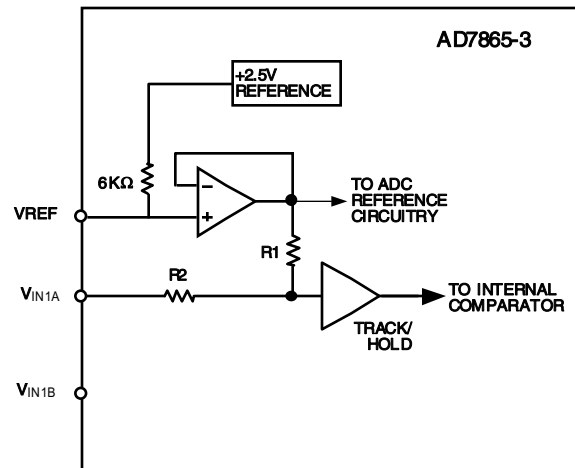
Figure 4. AD7865-3 Analog Input Structure
