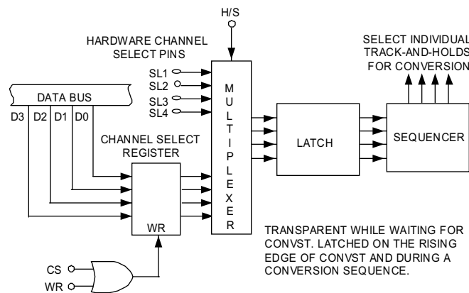
Figure 5. AD7865 Channel Select Inputs & Registers
