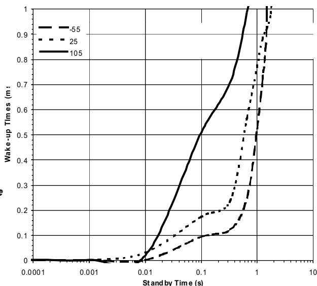
11. Power Up time Vs Standby Time using the On-Chip Reference
