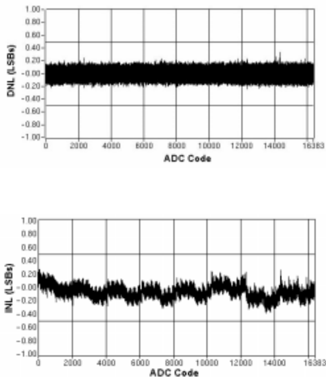
Figure 18. AD7865 Typical DNL and INL Plots
