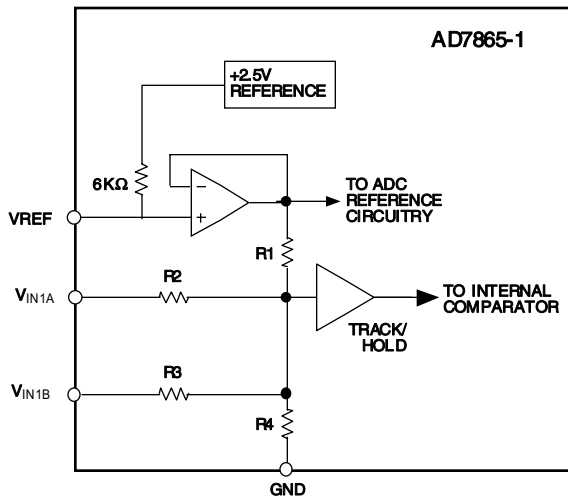
Figure 3. AD7865-1 Analog Input Structure
