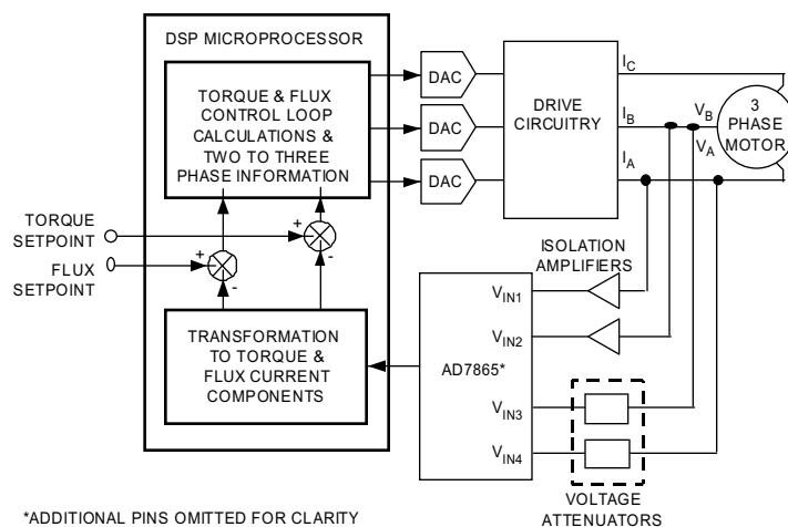
Figure 23. Vector Motor Control Using the AD7865.
