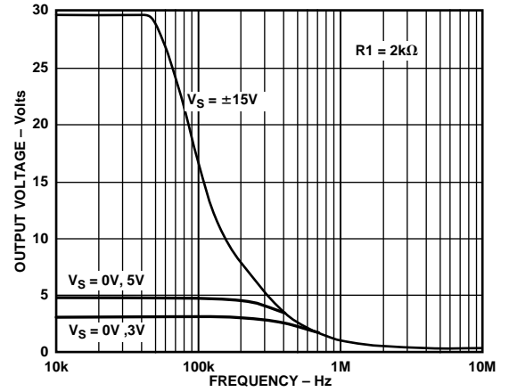
Figure 25. Large Signal Frequency Response
