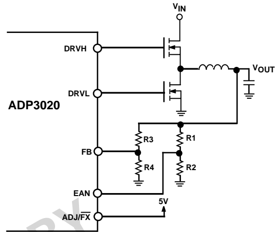
Figure 2. Adjustable Output Mode
