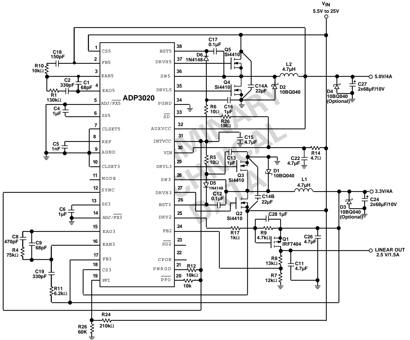
Figure 3. 45 W , Triple Output DC-DC Converter
