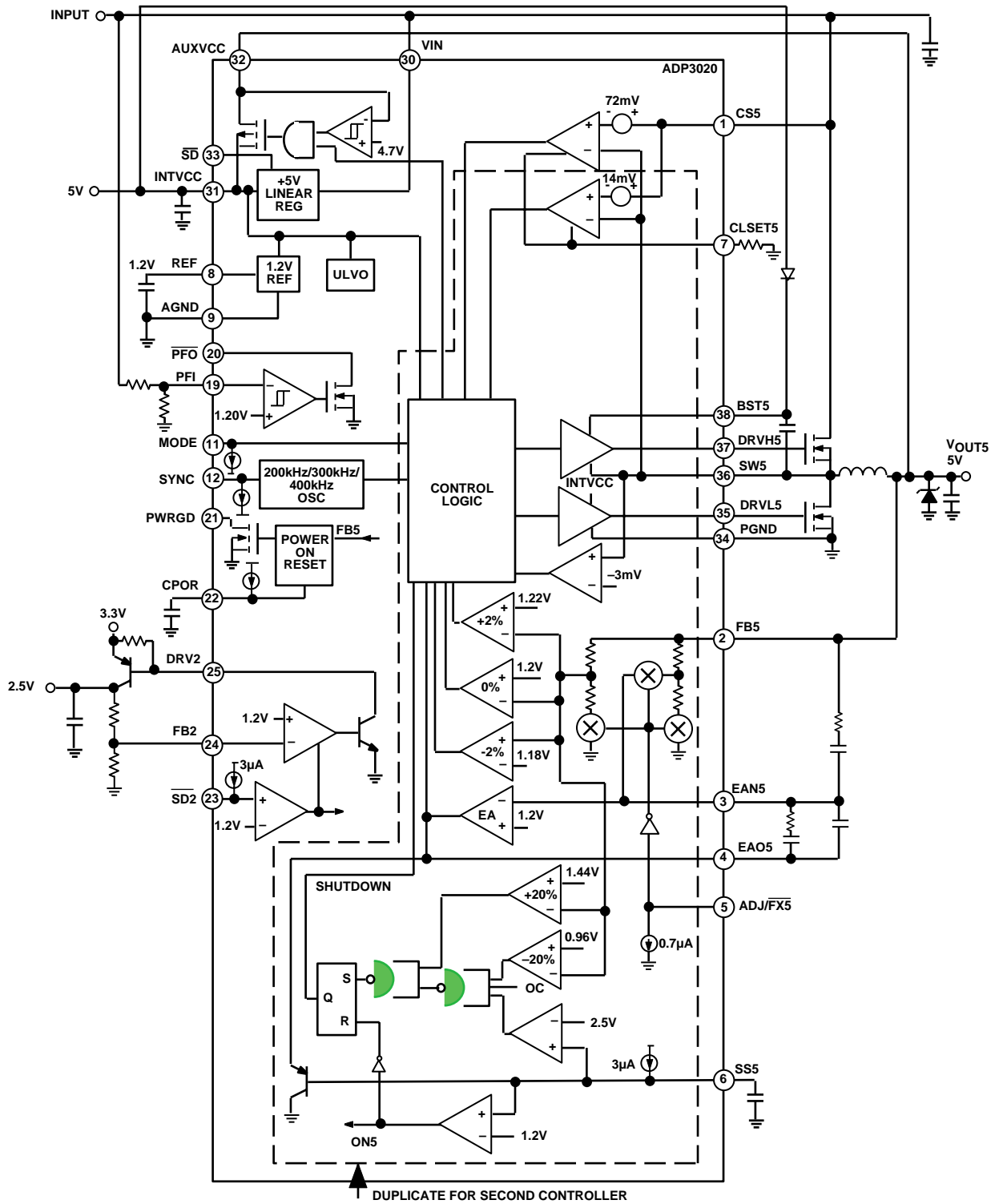
Figure 1. ADP3020 Block Diagram (Fixed Output Option)
