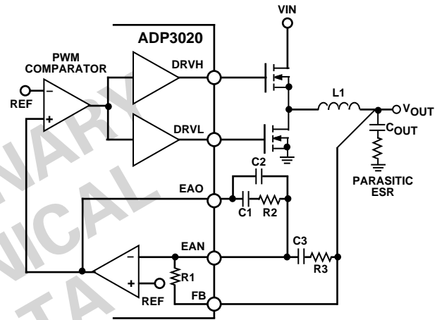
Figure 4. Buck Regulator Voltage Control Loop
