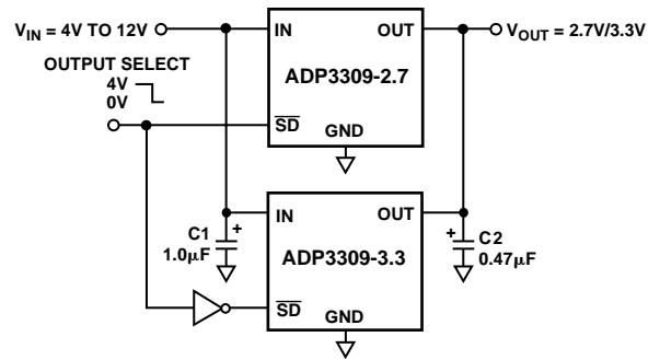
Figure 21. Crossover Switch
