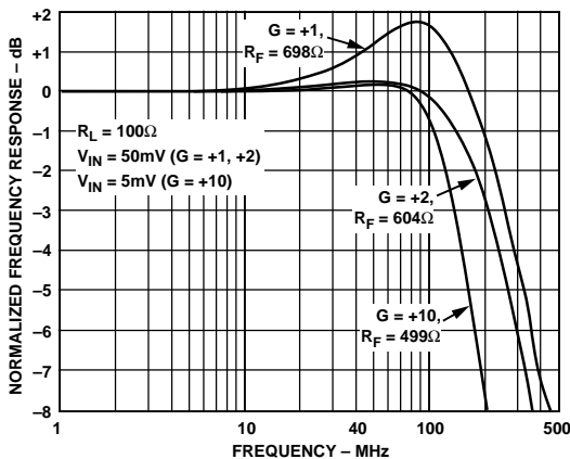
Figure 7. Frequency Response; G = +1, +2, +10 , V_S = \pm 5 V
