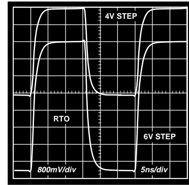
Figure 10.* Step Response; G = -2 , V_S = \pm 5 V
