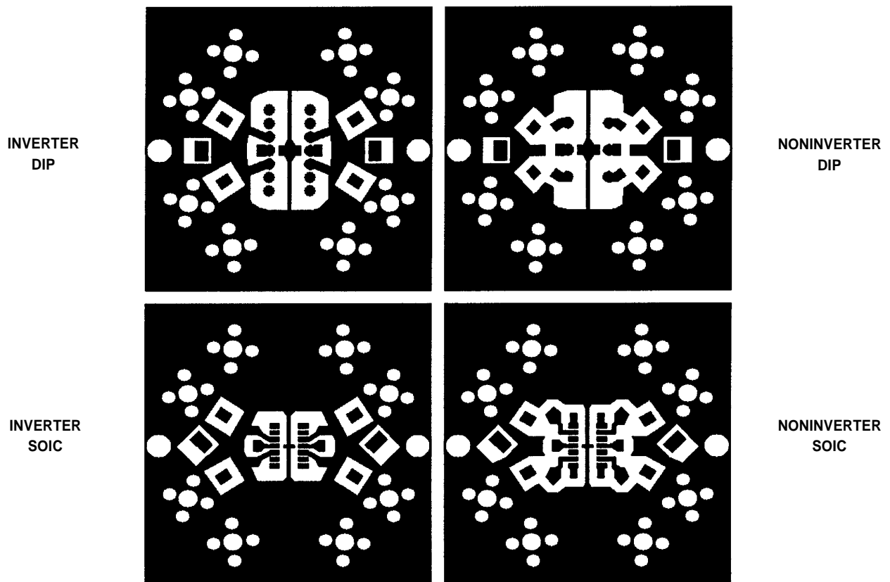
Figure 42. Evaluation Board Layout (Bottom Side, Looking Through the Board)
