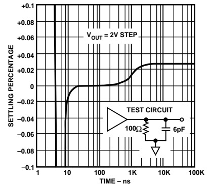
Figure 11. Long-Term Settling Time
