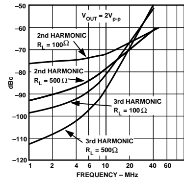
Figure 6. Harmonic Distortion vs. Frequency
