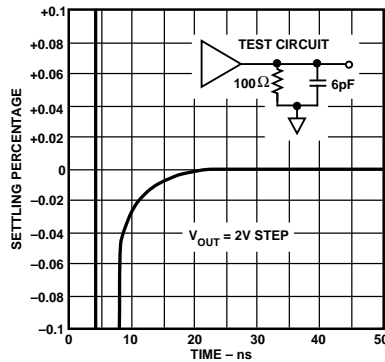
Figure 10. Short-Term Settling Time
