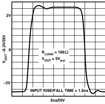
Figure 15. Large Signal Pulse Response
