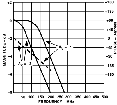
Figure 4. Inverting Frequency Response
