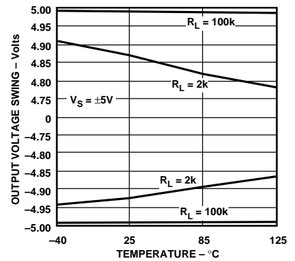
Figure 43. Output Voltage Swing vs. Temperature, V_S = \pm 5\text{ V}
