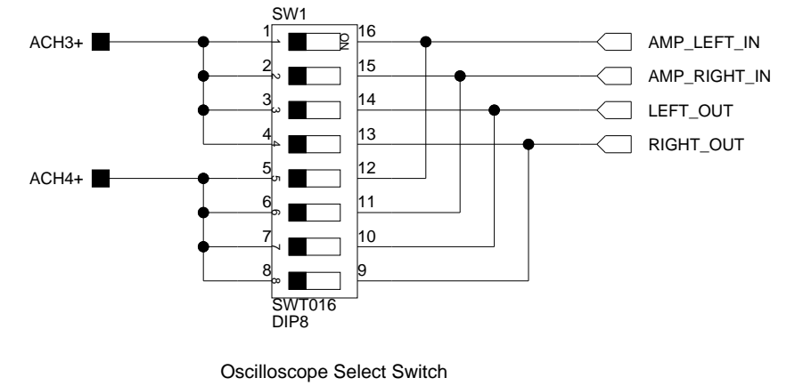
Oscilloscope Select Switch
